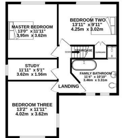
1ST FLOOR 668 sq.ft. (62.0 sq.m.) approx.
